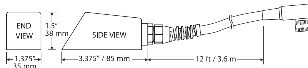
PSE4 ULTRASONIC DOPPLER SENSOR
